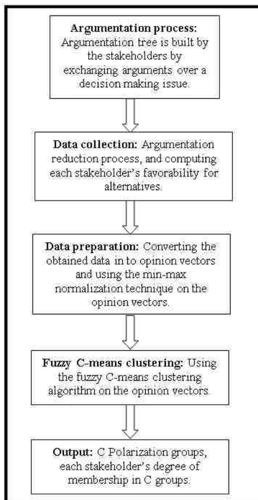
Figure 4.2. Fuzzy Based Polarization Assessment
