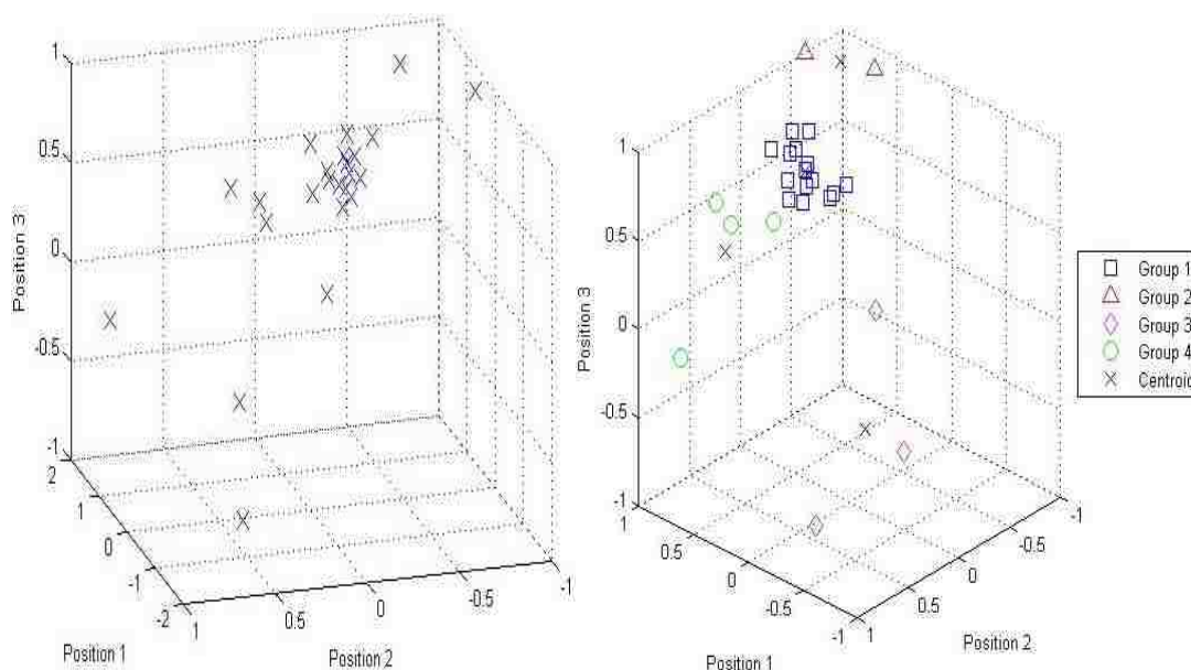
Figure 3.6a. Opinion Vectors before Polarization Assessment, Figure 3.6b. Polarization Groups Produced after Polarization Assessment
